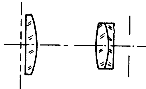
Kellner (K) \sim 40^\circ/45^\circ
